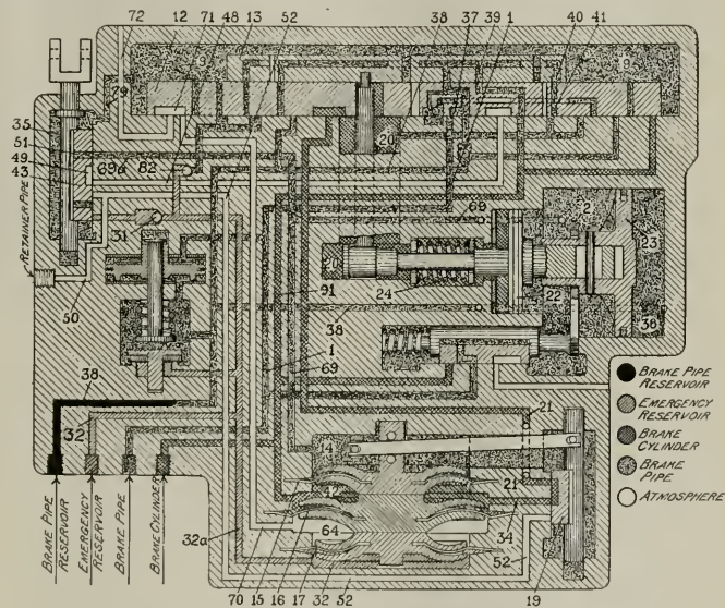
FIG. 5. SERVICE POSITION—TRIPLE VALVE IN GRADUATED RELEASE
